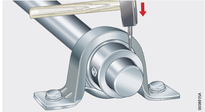
Figure 13 Tensioning the eccentric locking collar
