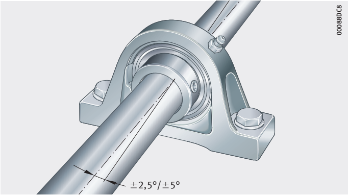
Figure 1 Compensation of static shaft misalignment
