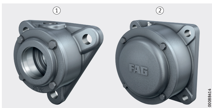
Figure 4 Flanged housings
