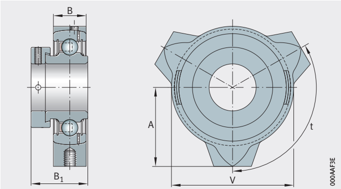
t = 120^\circ Figure 1 Take-up housing unit as hanger bearing for ventilators Possible combinations
