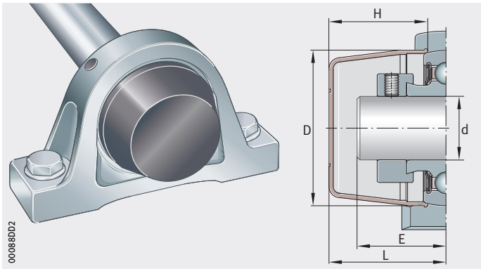
Figure 6 Housing unit with bearing end cap
