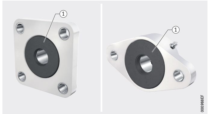
Figure 2 Flanged housing units with Back Seal component
